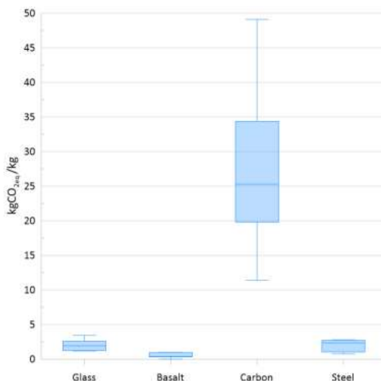
Figure 22 Distribution of collected values of kgCO_{2eq}/kg of fibres.
